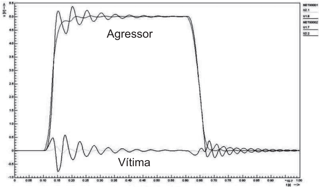
Crosstalk Simulation Result
